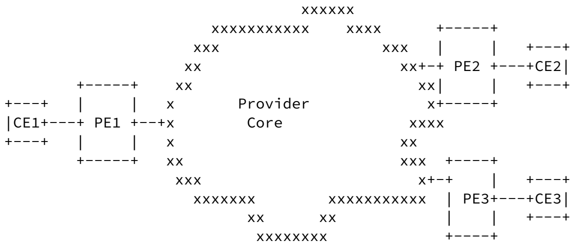
MVPN topology
