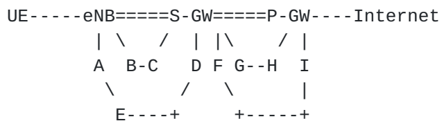
Figure 3 LTE nodes connected to multi-paths via IP transport nodes
