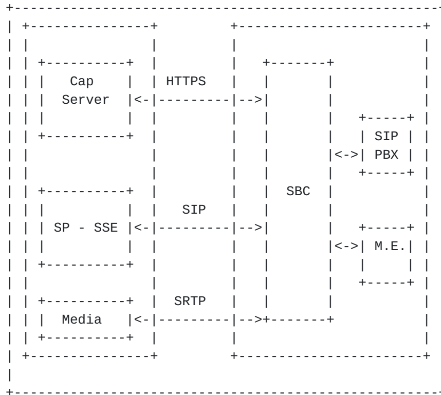
Figure 1: Reference Architecture
