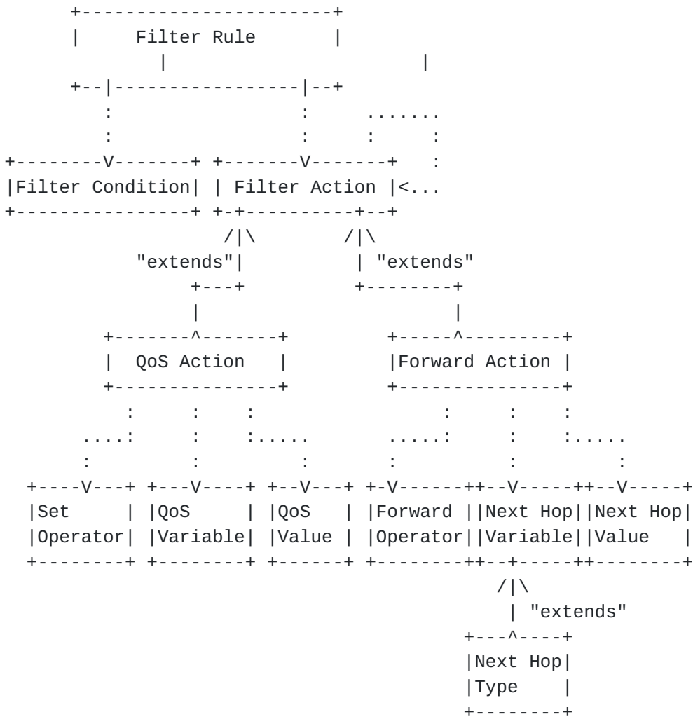
Figure 5: Filter Actions for FB-RIB
