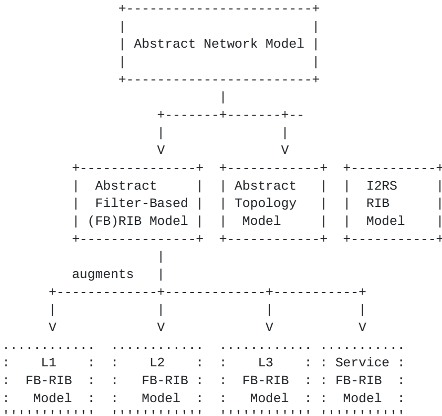
Figure 1: The network model structure
