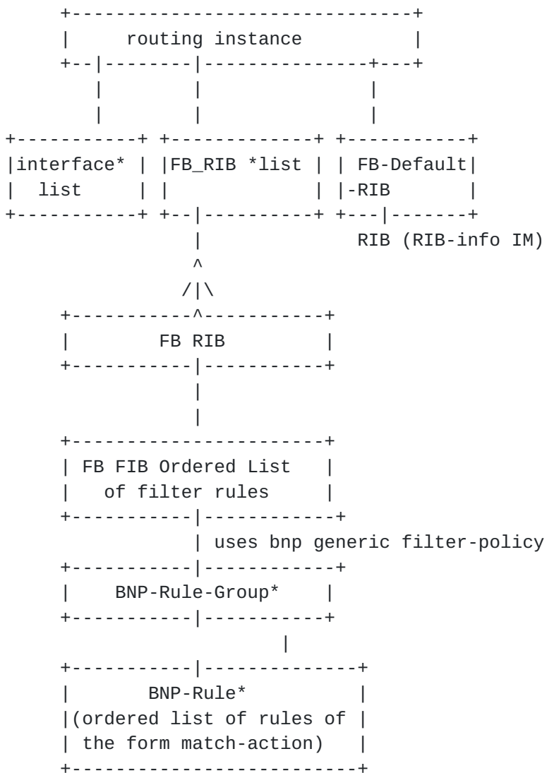
Figure 4: Routing instance with FB-RIB
