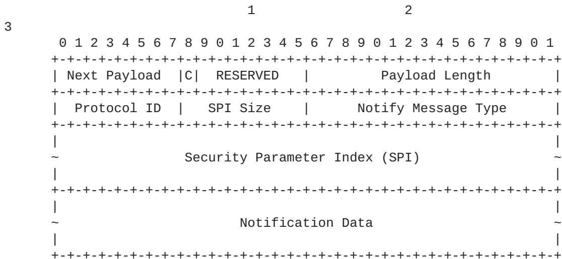
Figure 3: Notify Payload Format.
