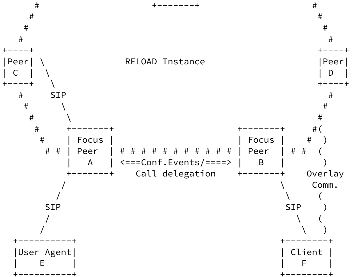
Figure 1: Reference Scenario: Focus peers A,B maintain a distributed conference
