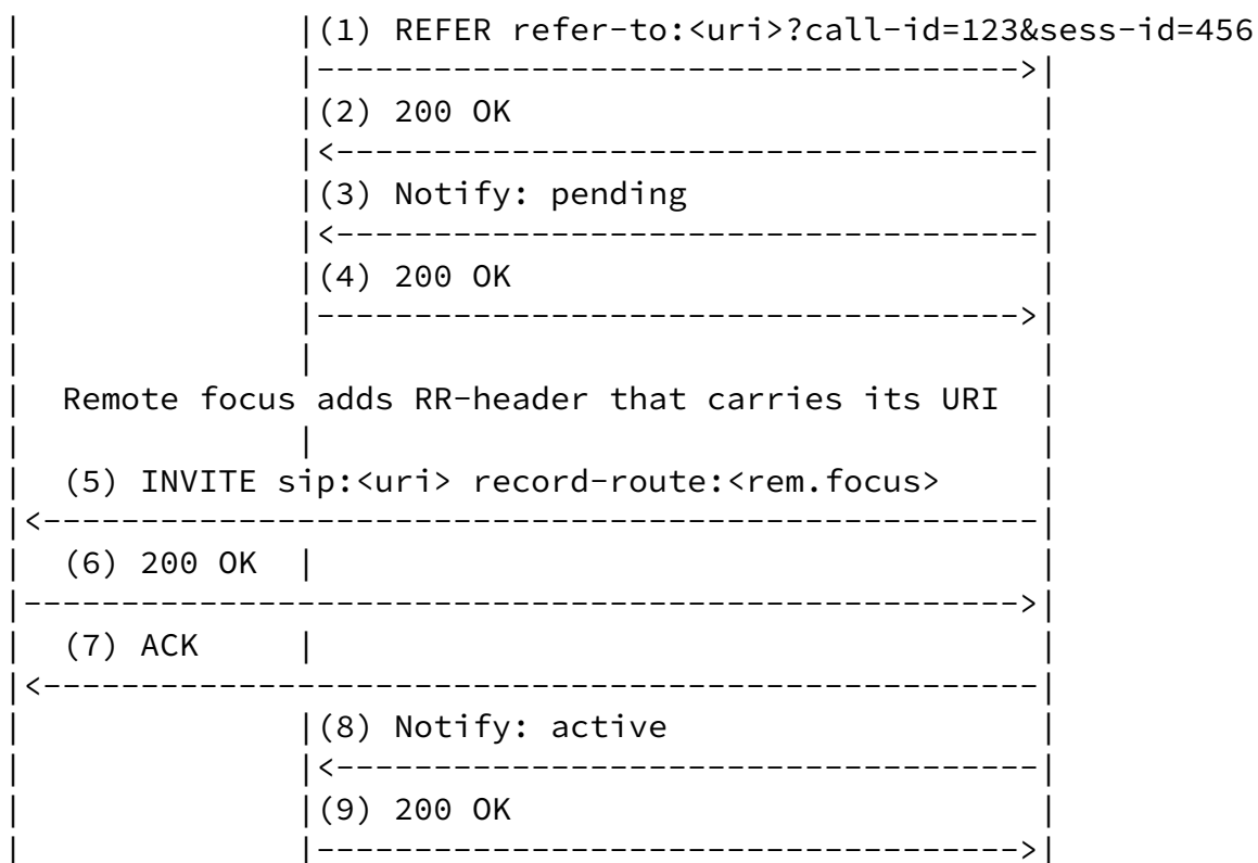
Figure 6: Delegating a participant with SIP REFER
