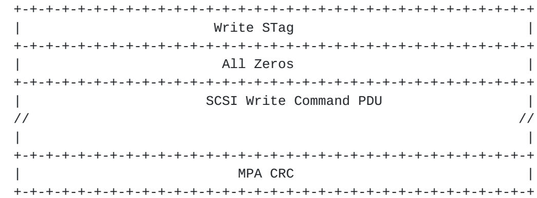
Figure 10 SendSE Message containing a SCSI Write Command PDU
