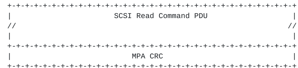
Figure 8 SendSE Message containing a SCSI Read Command PDU
