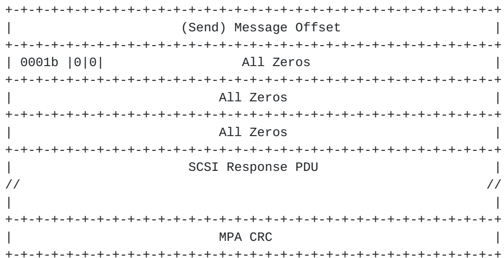
Figure 13 SendInvSE Message containing SCSI Response PDU
