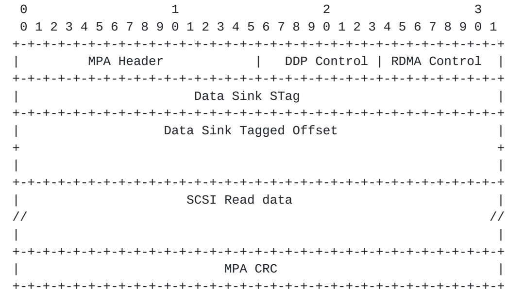
Figure 9 RDMA Write Message containing SCSI Read Data
