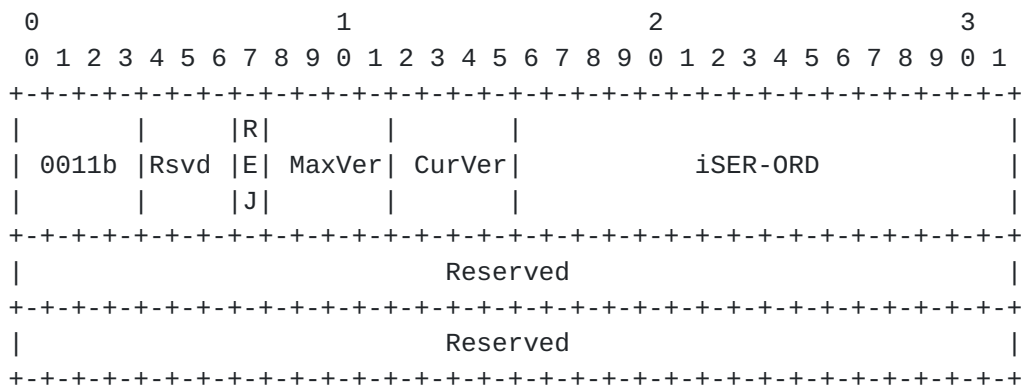
Figure 5 iSER Header Format for iSER HelloReply Message
