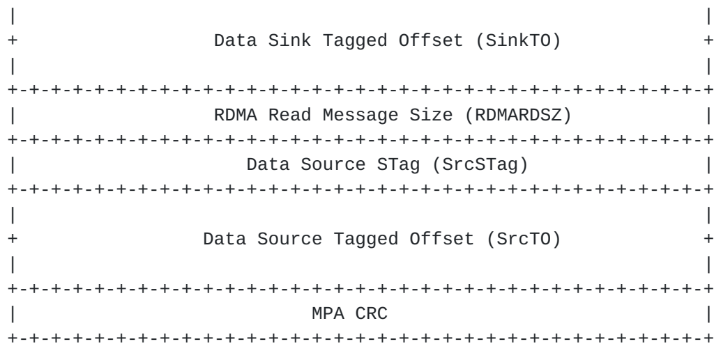
Figure 11 RDMA Read Request Message
