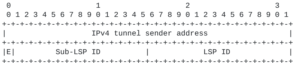
Figure 3: MLSP_TUNNEL_IPv4 Sender Template
