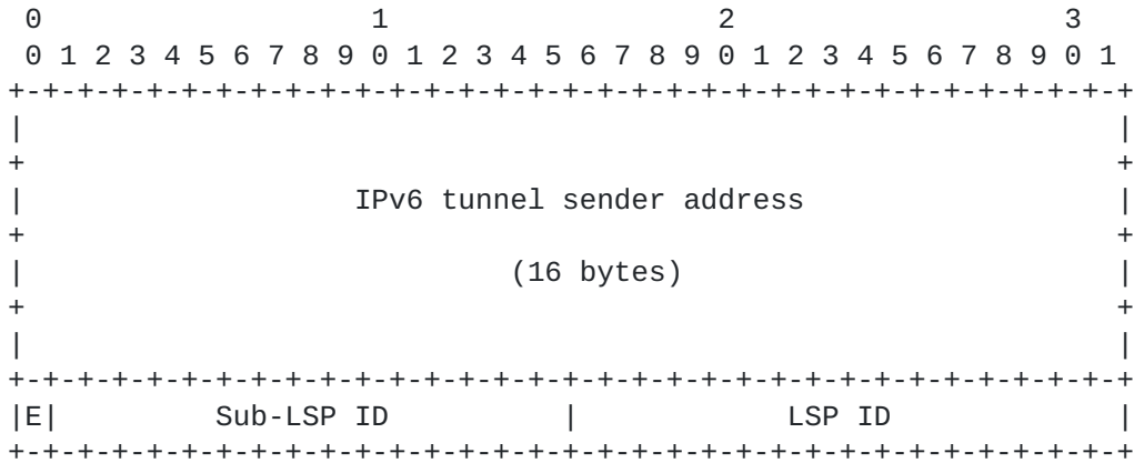
Figure 4: MLSP_TUNNEL_IPv6 Sender Template
