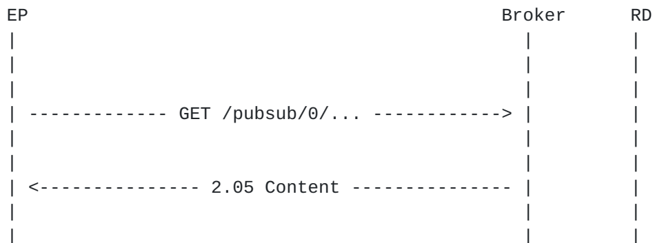
Figure 6: Client EP GET from CoAP-PubSub Broker
