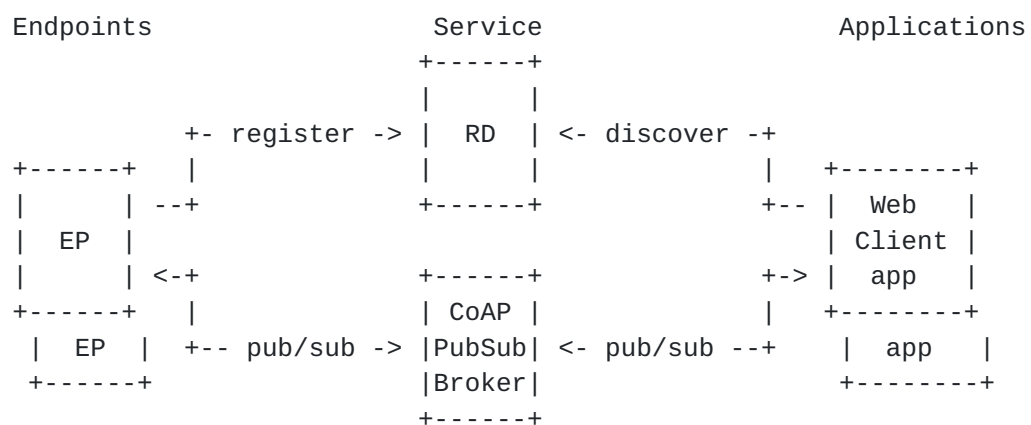
Figure 1: CoAP-PubSub Architecture
