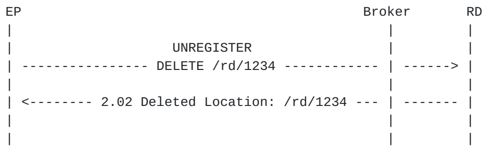
Figure 3: Unregister Endpoint
