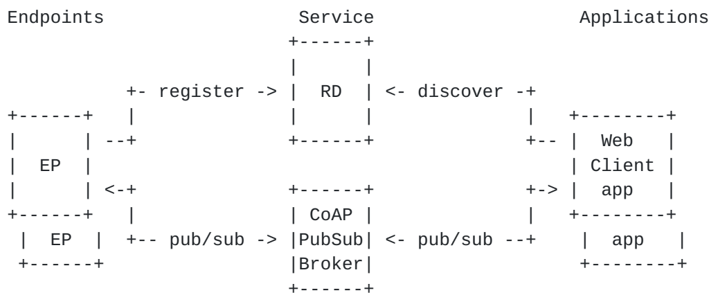
Figure 1: CoAP-PubSub Architecture
