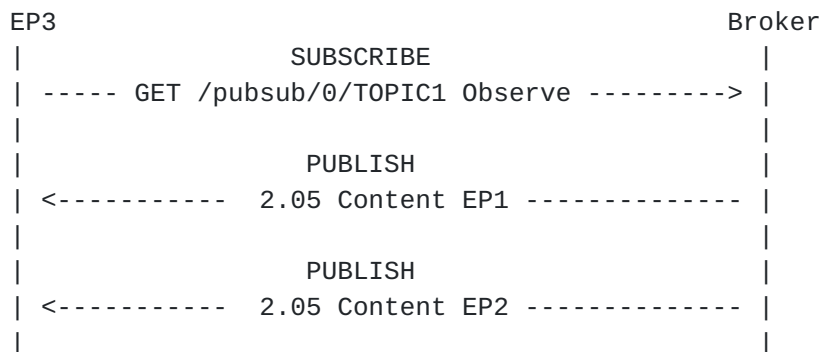
Figure 11: CoAP-PubSub Endpoint SUBSCRIBE to Broker
