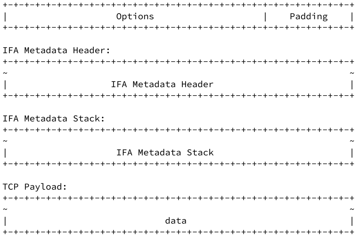
Figure 8: TCP/UDP IFA Packet Format
