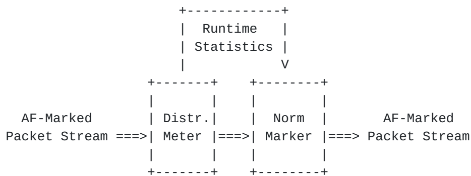
Normalization Marker (NM) with AF PHB Group
