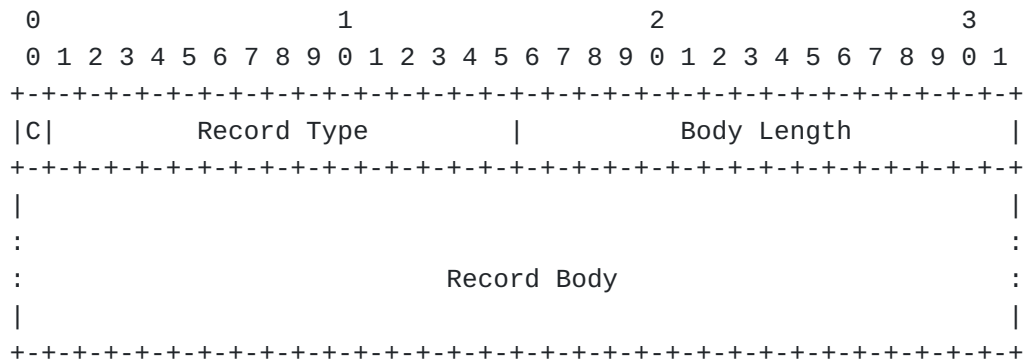
Figure 6: NTS-KE record format
