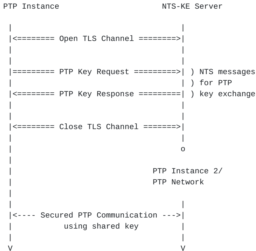
Figure 1: NTS key distribution sequence
