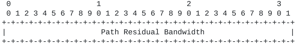
Figure 1: PATH RESIDUAL BANDWIDTH value format
