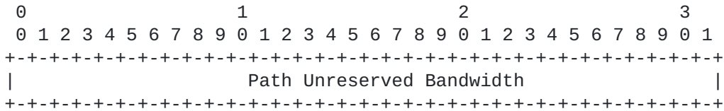
Figure 1: PATH UNRESERVED BANDWIDTH value format
