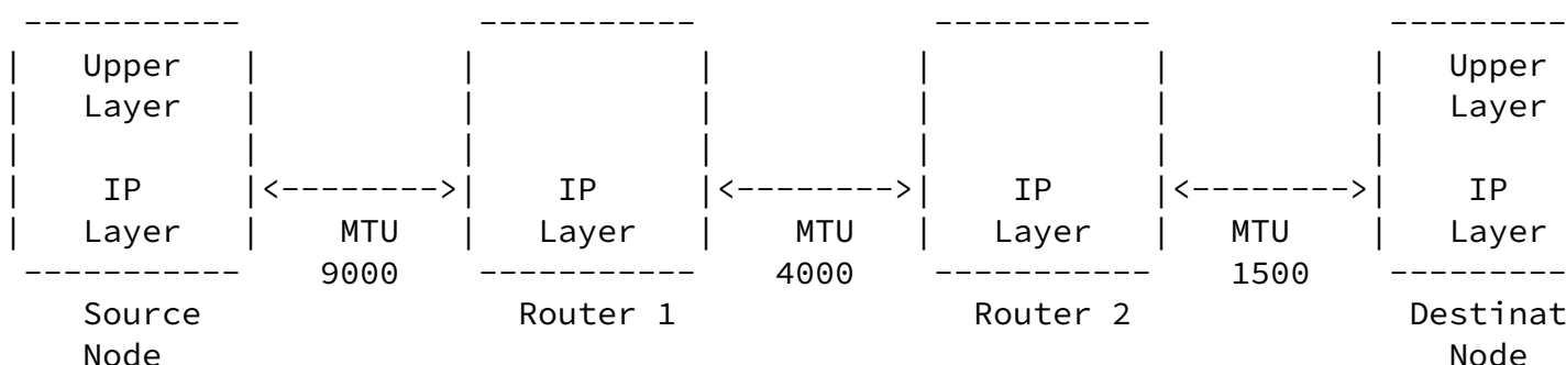
Figure 1: Reference Topology
