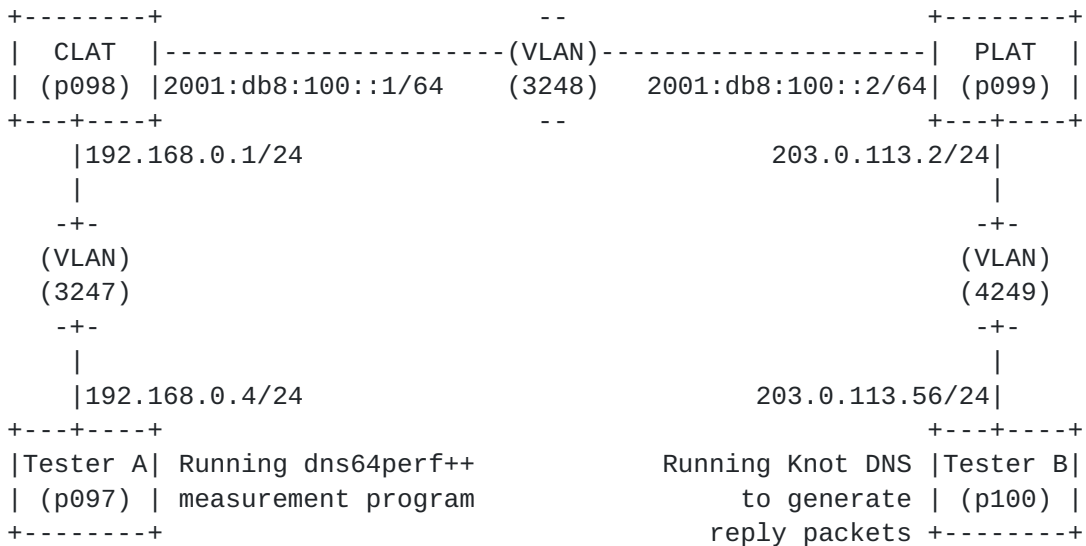
Figure 12: Test setup for benchmarking 464XLAT using DNS traffic
