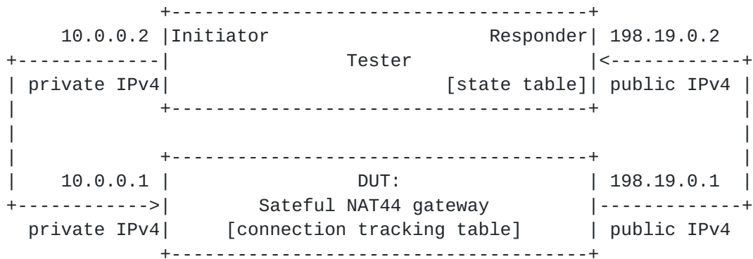
Figure 1: Test setup for benchmarking stateful NAT44 gateways
