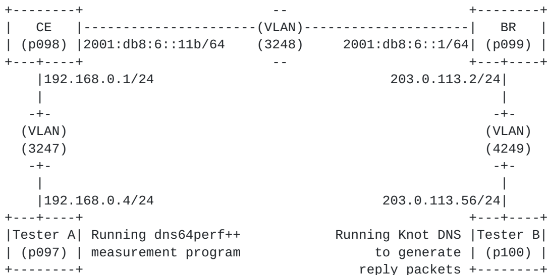
Figure 14: Test setup for benchmarking MAP-T using DNS traffic
