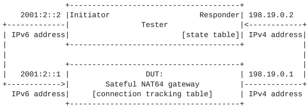
Figure 7: Test setup for benchmarking stateful NAT64 gateways
