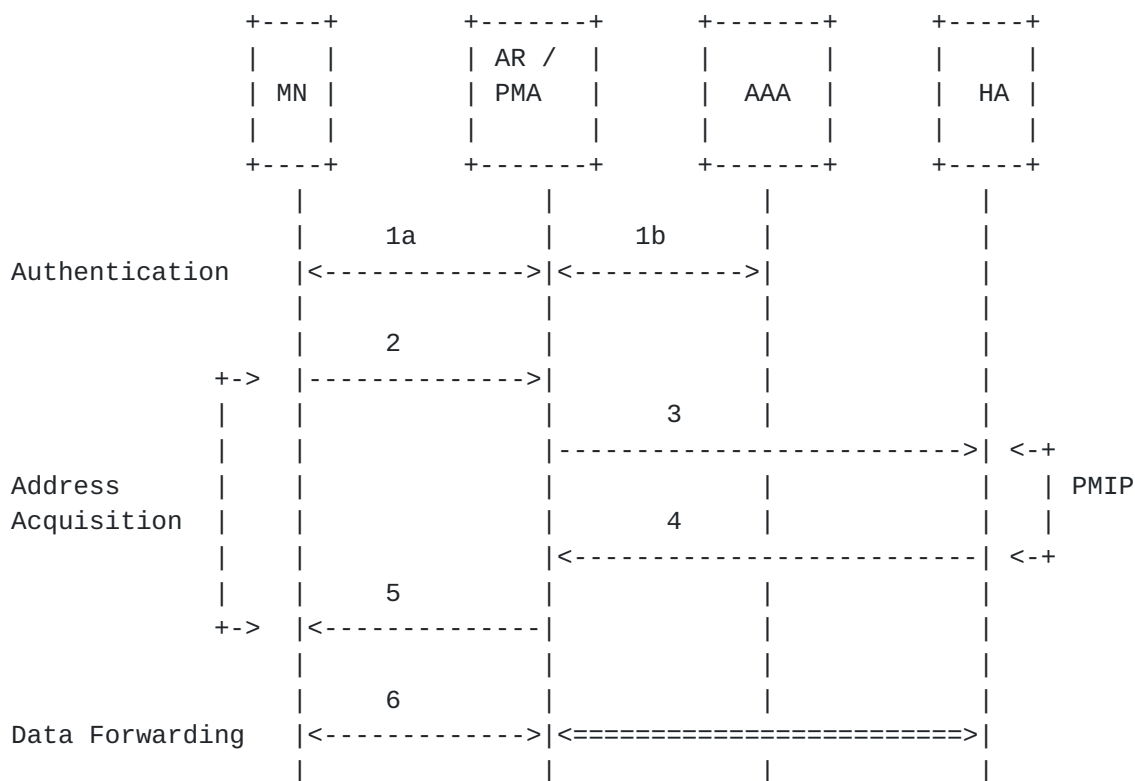
Figure 1: Network Connection Setup
