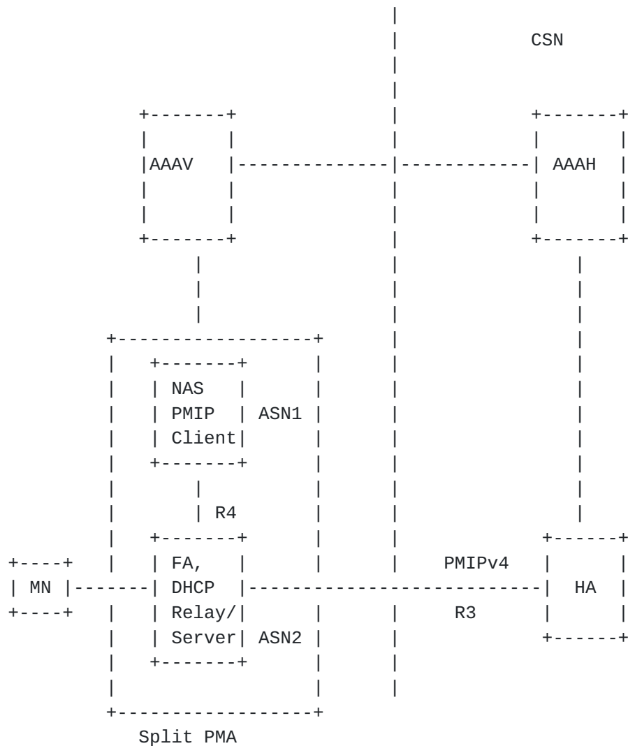
WiMAX NWG network configuration for PMIP use
