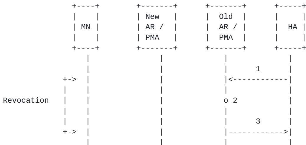
Figure 4: Registration Revocation for Previous PMA
