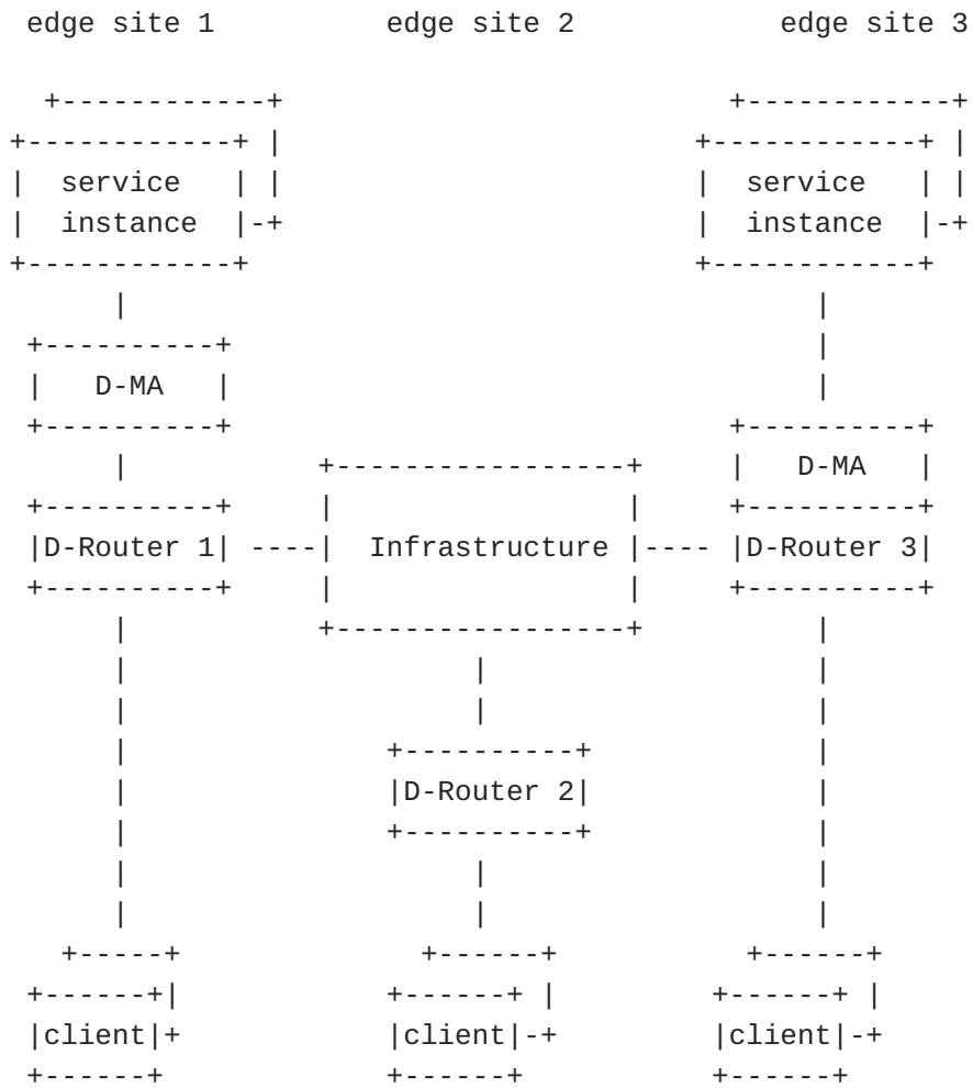
Figure 1: Dyncast Architecture.
