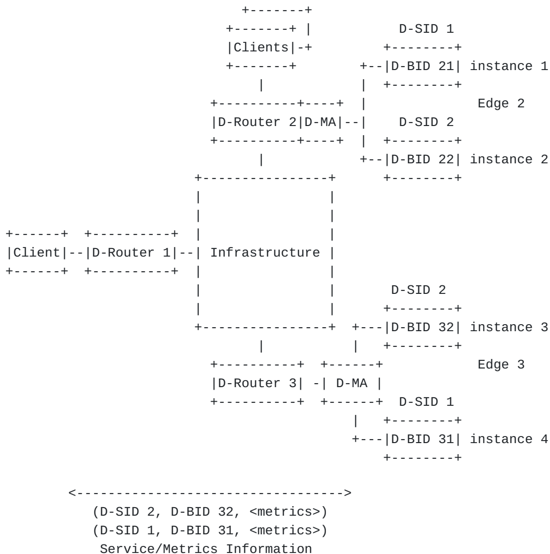
Figure 2: Dyncast deployment example.
