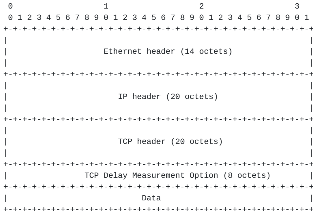
Figure 4: Figure 4: Format of Reference or Target Packet
