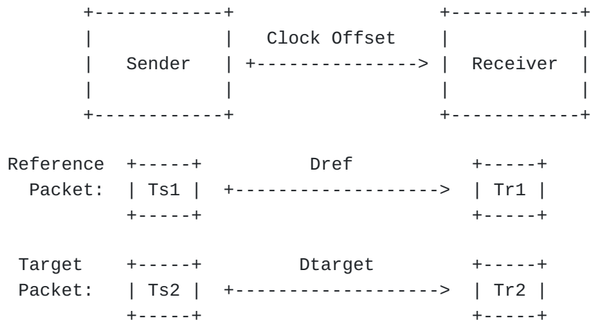
Figure 2: Figure 2:Topology of One-way Delay Measurement
