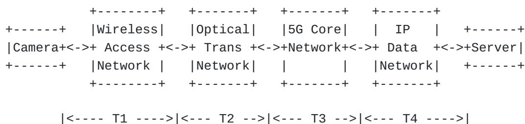
Figure 1: Figure 1:A Scenario for End-to-end One-way Delay
