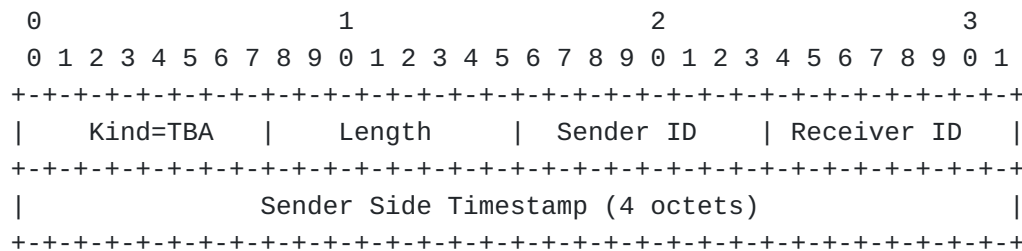
Figure 5: Figure 5: TCP Delay Measurement Option Format
