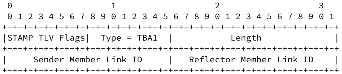
Figure 2: LAG Member Link ID TLV
