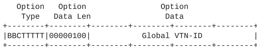
Figure 2. The format of Global VTN-ID Option
