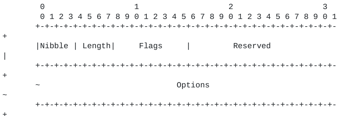
Figure 1. The format of VTN extension header
