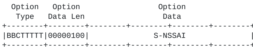
Figure 3. The format of 5G network slice ID Option
