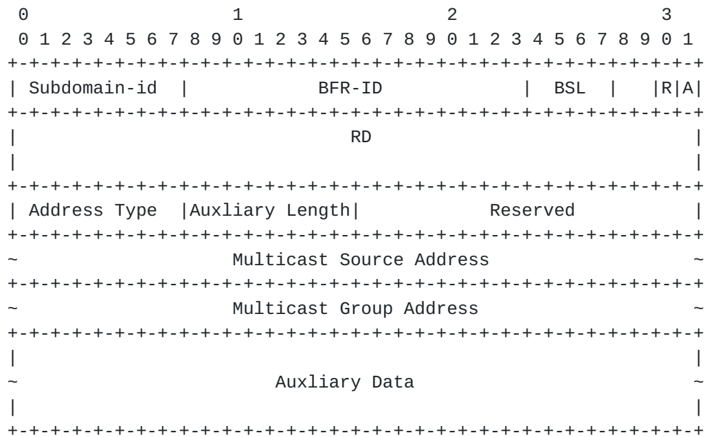
Figure 2: MSR Object Body Format
