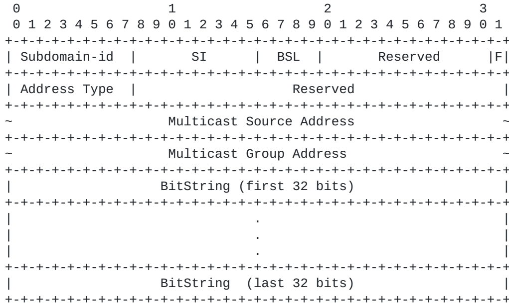
Figure 4: FI Object Body Format
