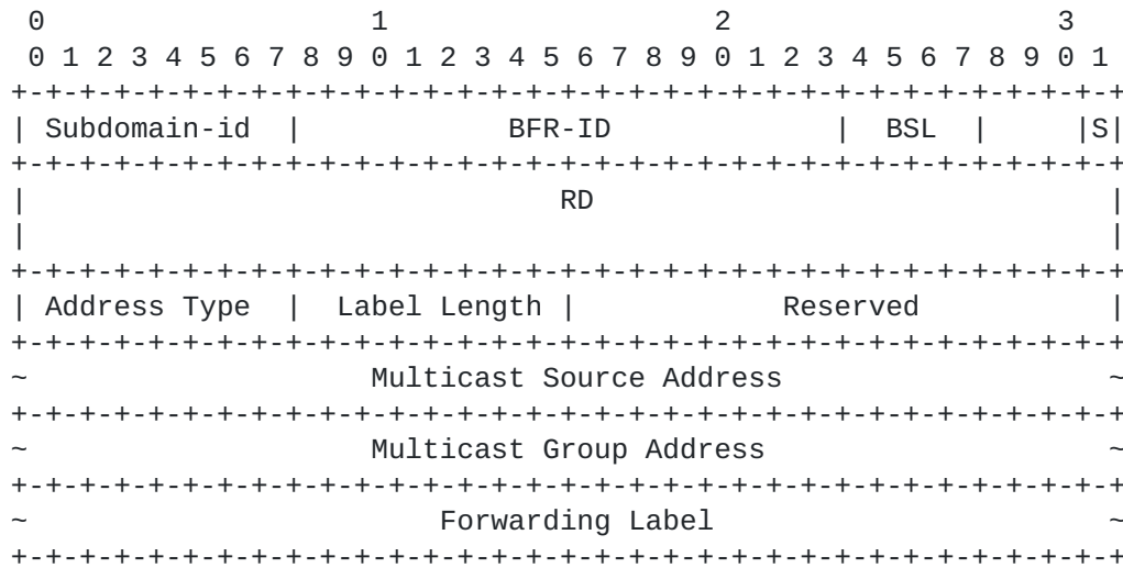
Figure 3: MRI Object Body Format
