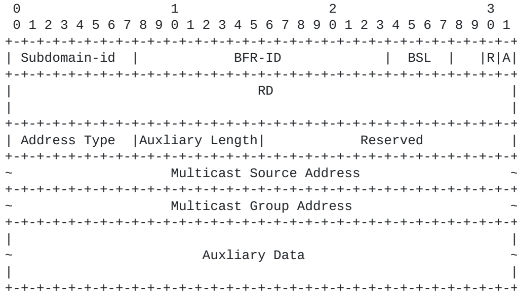
Figure 2: MSR Object Body Format
