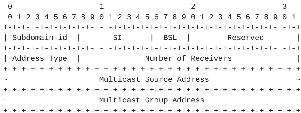
Figure 5: MRS Object Body Format
