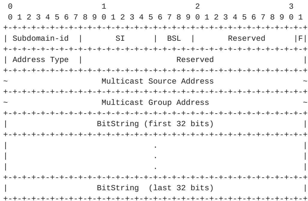
Figure 4: FI Object Body Format
