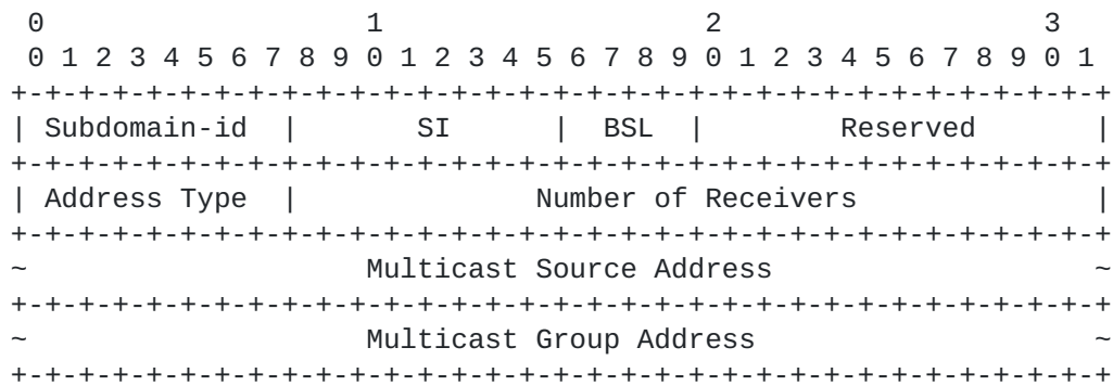
Figure 5: MRS Object Body Format
