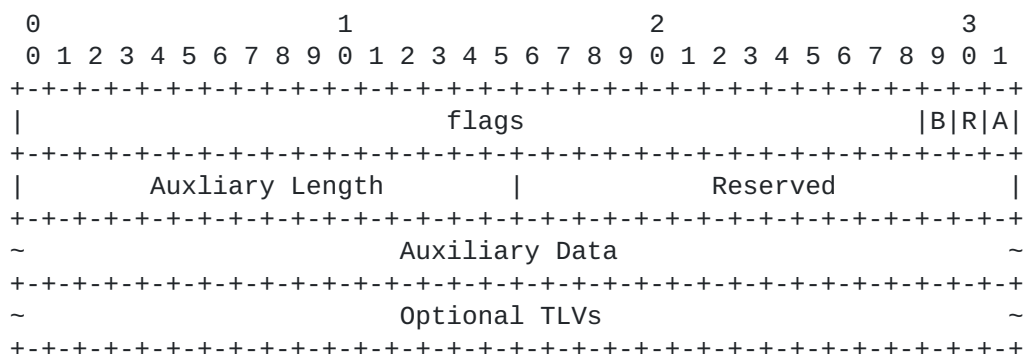
Figure 2: MSR Object Body Format
