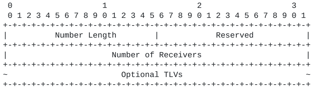
Figure 9: MRS Object Body Format
