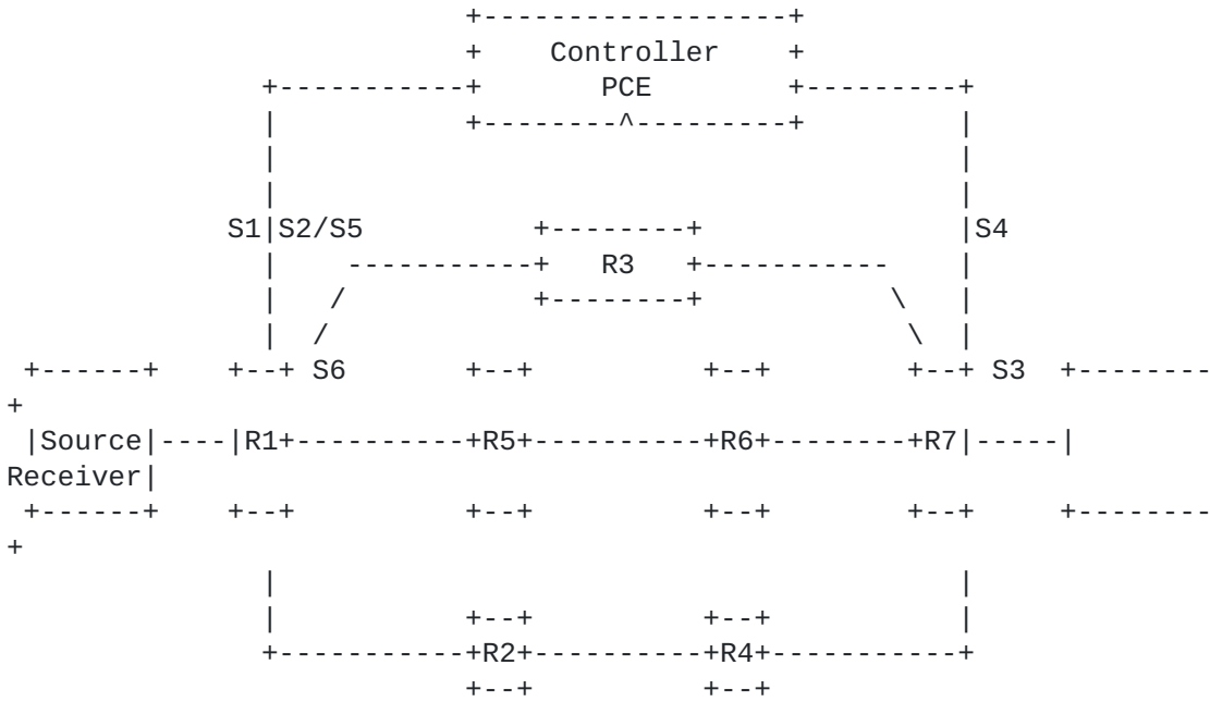
Figure 1: Example of PCE based BIER Topology(controller as PCE)
