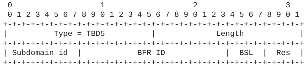
Figure 4: BIER Information TLV Format
