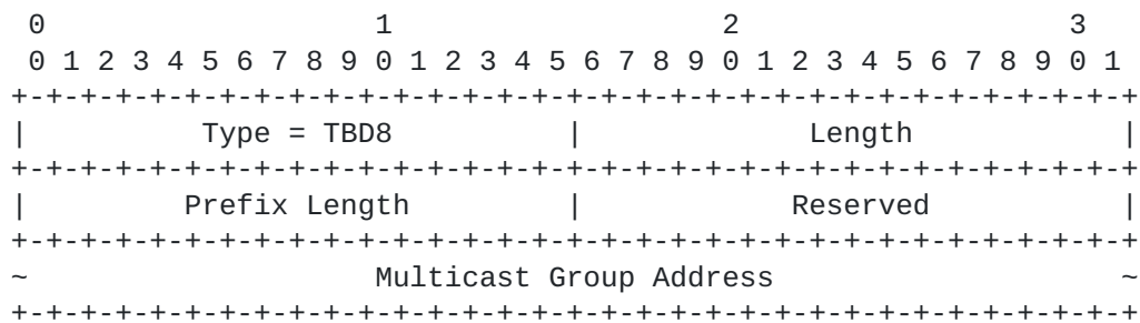
Figure 7: Multicast Group Address TLV Format
