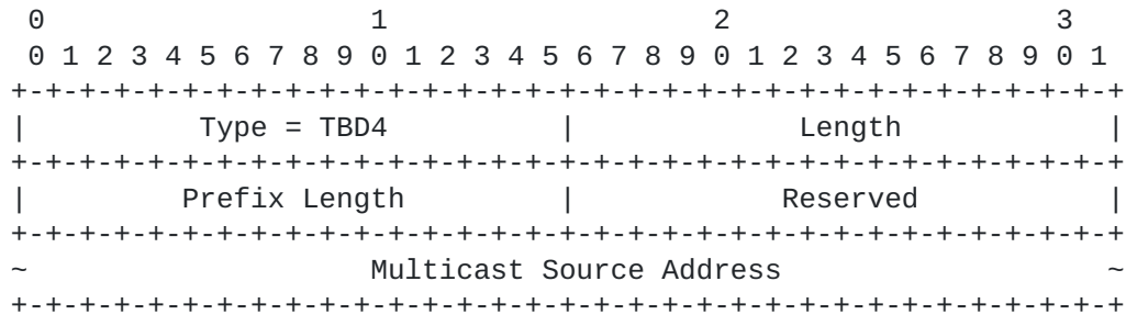
Figure 3: Multicast Source Address TLV Format
