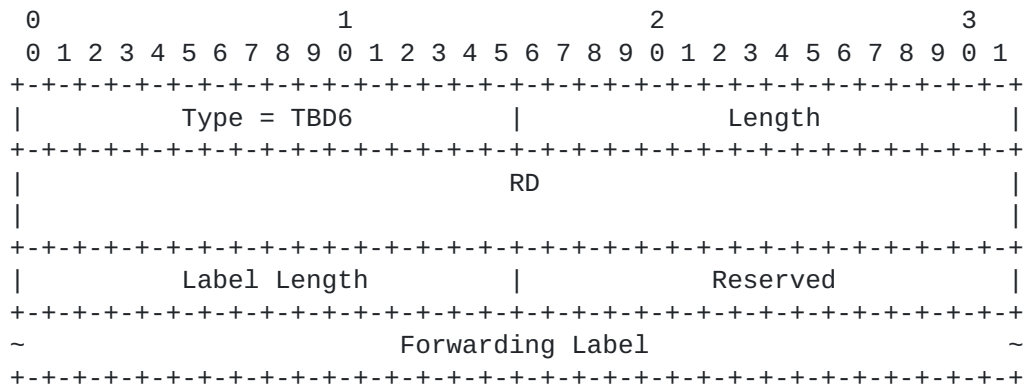
Figure 5: VPN Information TLV Format
