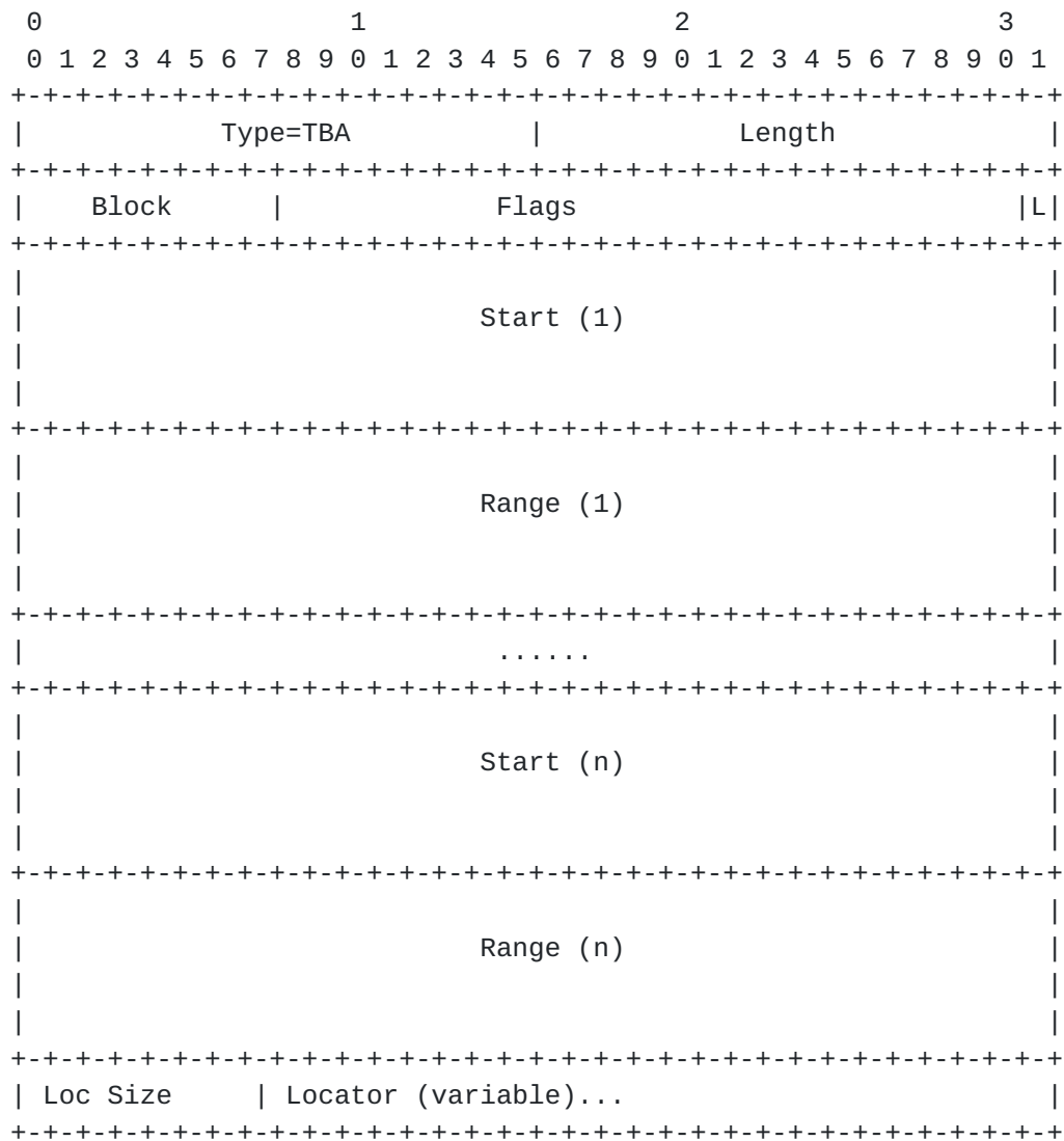
Figure 3: FUNCT-ID-CONTROL-SPACE TLV
