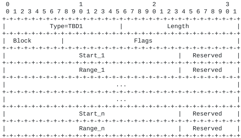
Figure 2: LABEL-CONTROL-SPACE TLV
