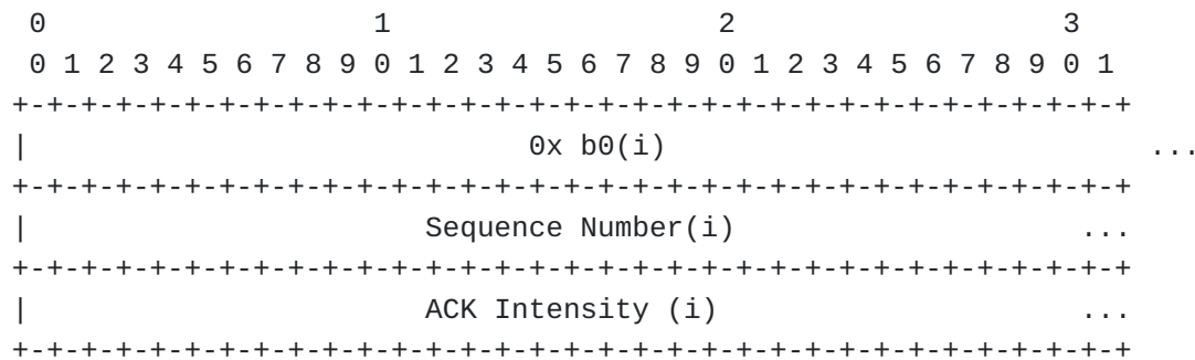
Figure 1: ACK-INTENSITY Frame
