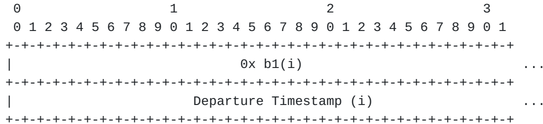
Figure 2: TIMESTAMP Frame
