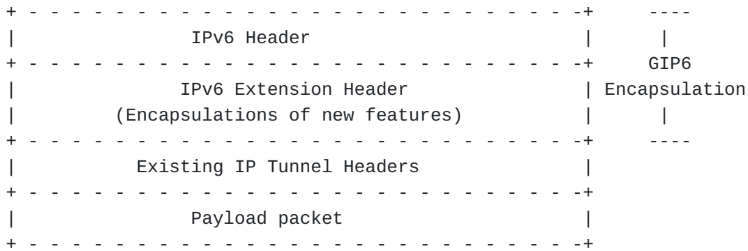
Figure 2. GIP6 Encapsulation with Existing IP Tunnel Headers
