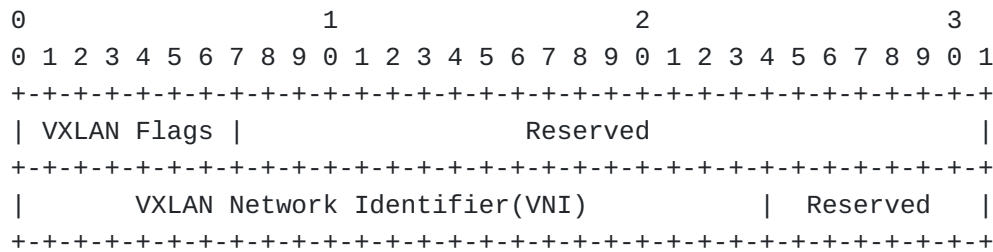
Figure 4. VXLAN headers
