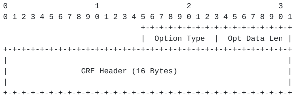
Figure 5. GRE Option
