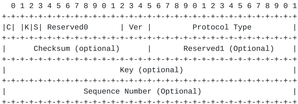
Figure 6. GRE Header
