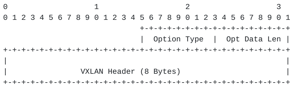
Figure 3. VN Option
