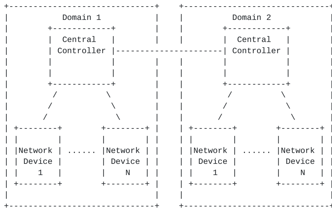
Figure 1: An Architecture of Network Artificial Intelligence(NAI)
