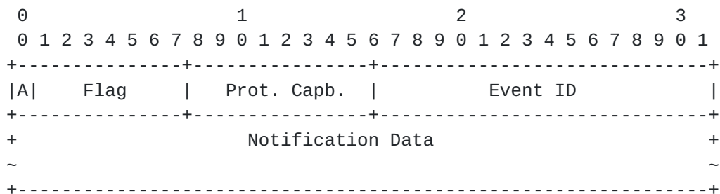
Figure 6. PASP Notification Message
