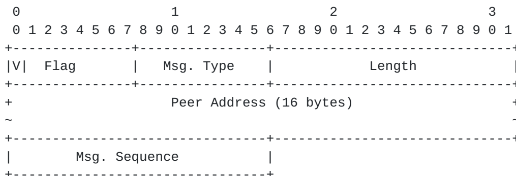
Figure 2. PASP Common Header
