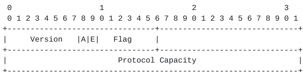
Figure 3. PASP Negotiation Message
