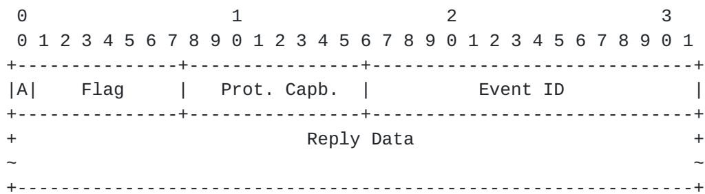
Figure 5. PASP Reply Message
