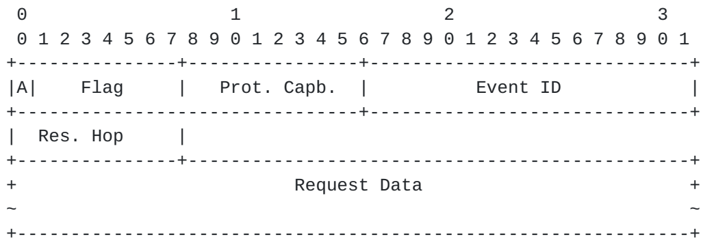
Figure 4. PASP Request Message
