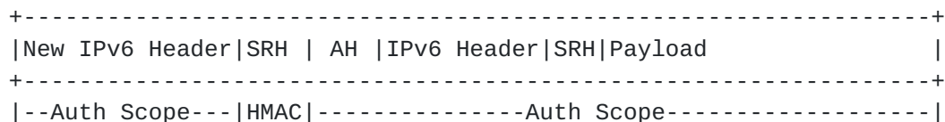
Figure 3: Transport Mode AH and HMAC for SRV6 packets
