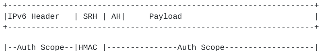
Figure 3: Transport Mode AH and HMAC for SRV6 packets
