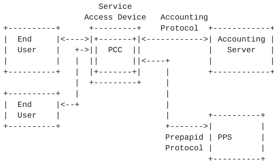
Figure 1: Basic Prepaid Architecture
