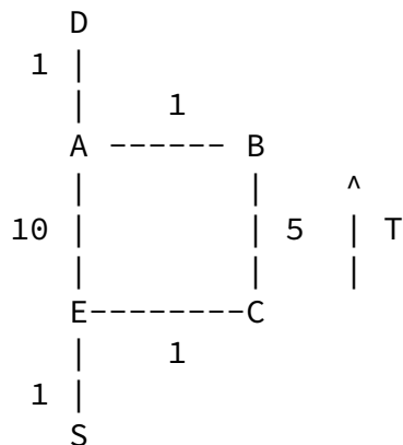
Figure 2 - RSVPTE FRR case
