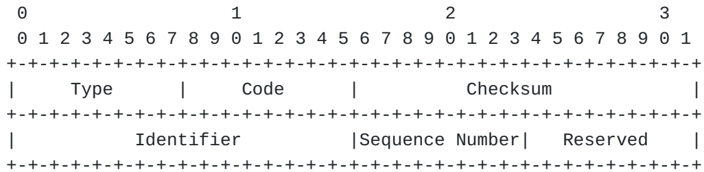
Figure 3: Validation Reply
