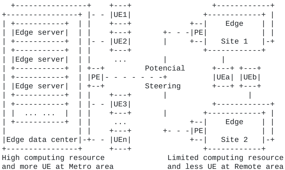
Figure 1: Common Deployment of Edge Sites
