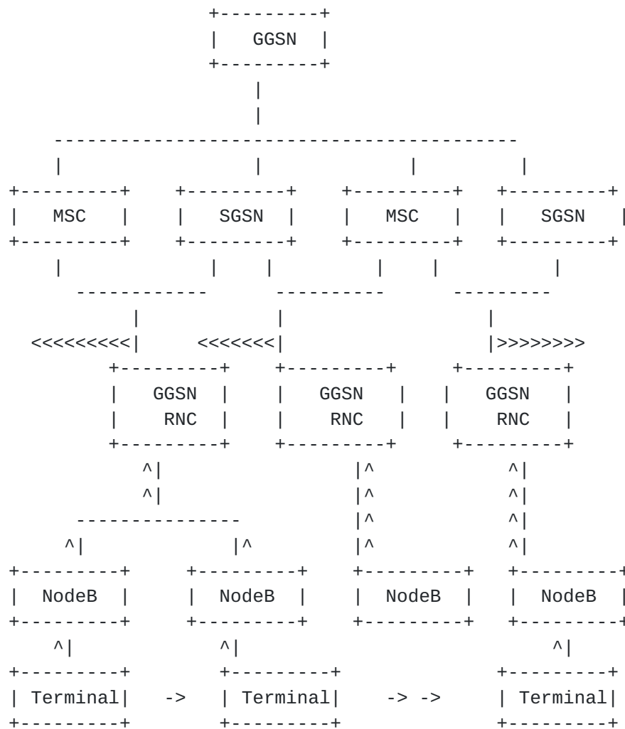
Figure 3 SIPTO Scenario
