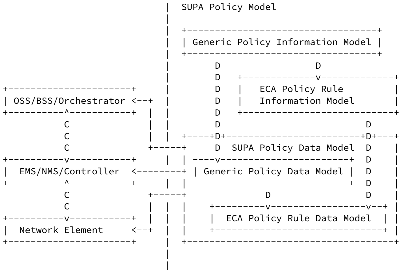
Figure 2: SUPA Policy Model Framework
