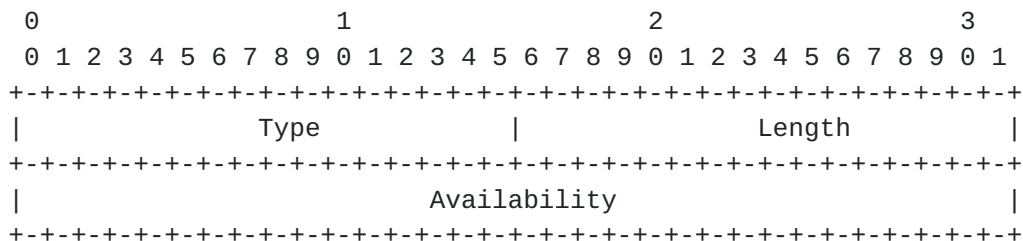
Figure 2: Availability sub-TLV
