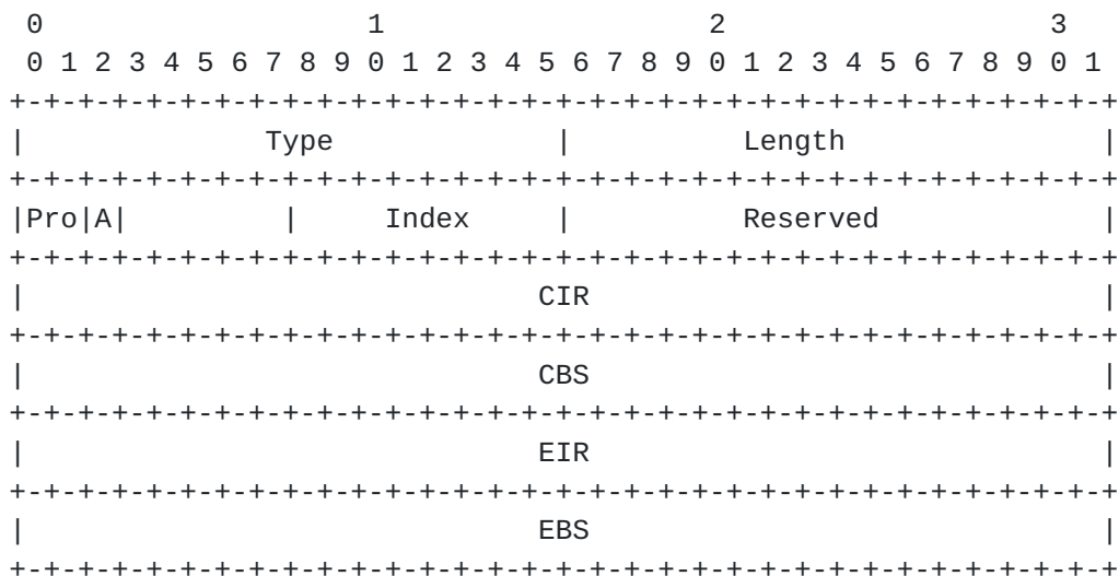
Figure 1: A new "AF" field in Ethernet Bandwidth Profile TLV
