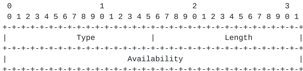
Figure 2: Availability sub-TLV
