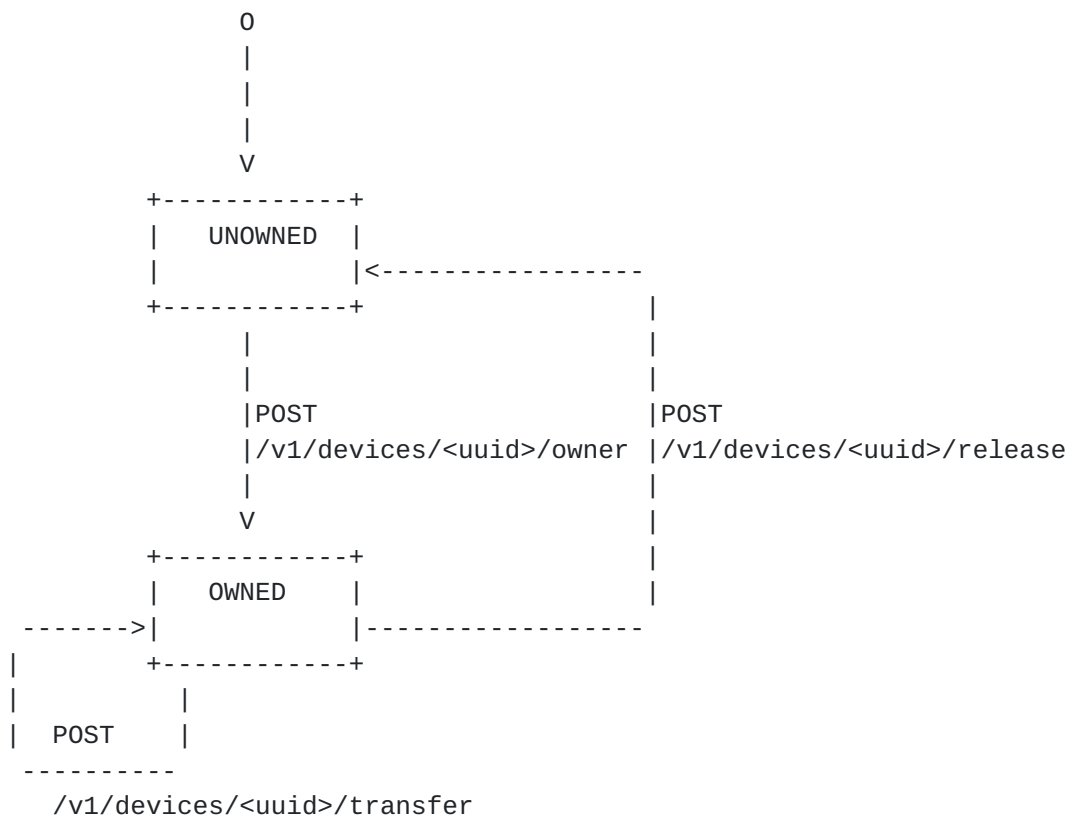
Device Ownership State Machine
