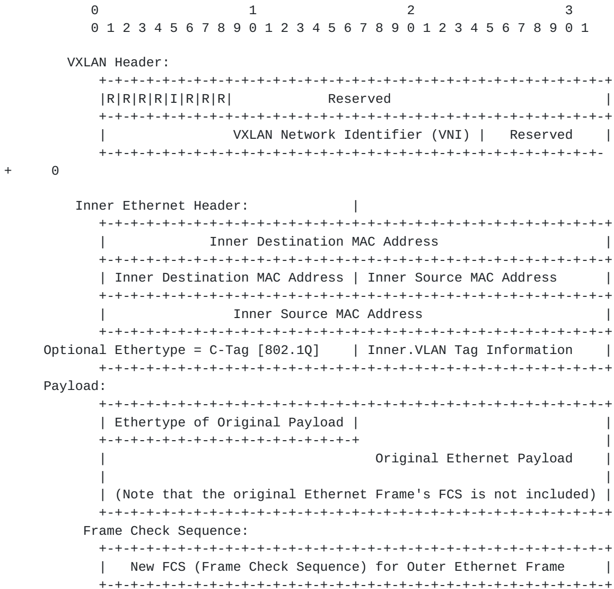
Figure 1 VXLAN Frame Format
