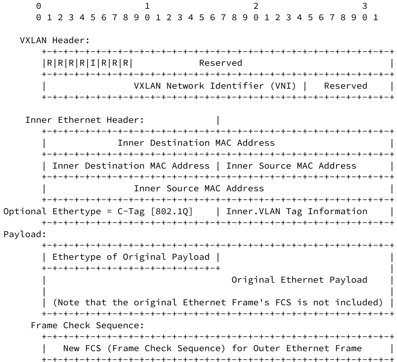
Figure 1 VXLAN Frame Format
