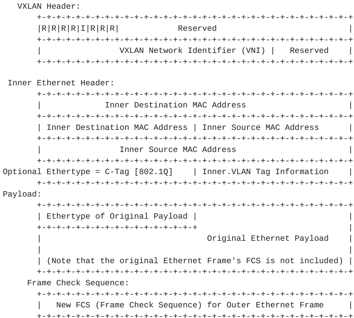
Figure 2 VXLAN Frame Format with IPv6 Outer Header
