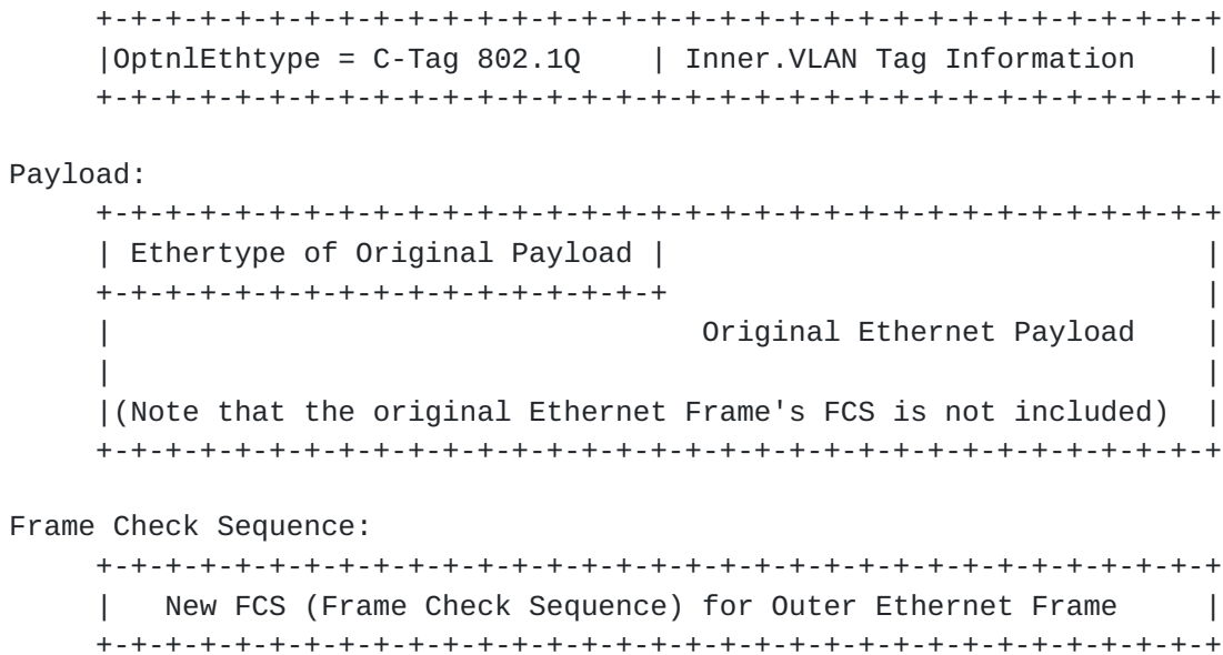
Figure 2 VXLAN Frame Format with IPv6 Outer Header
