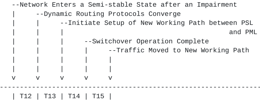
Figure 3. Dynamic Rerouting Cycle Model
