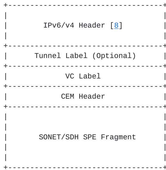
Figure 4. MPLS Transport Encapsulation
