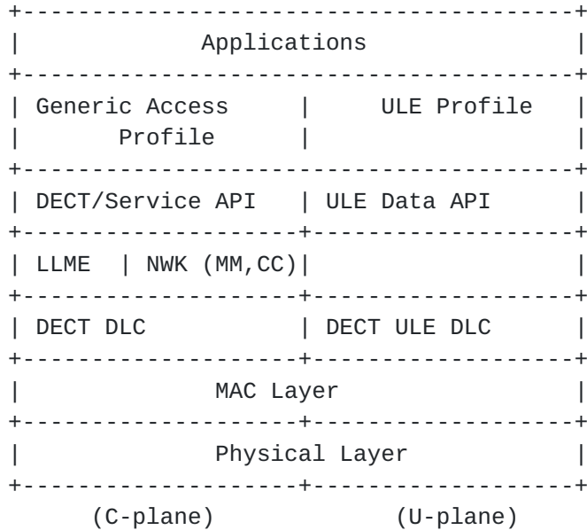
Figure 1: DECT ULE Protocol Stack
