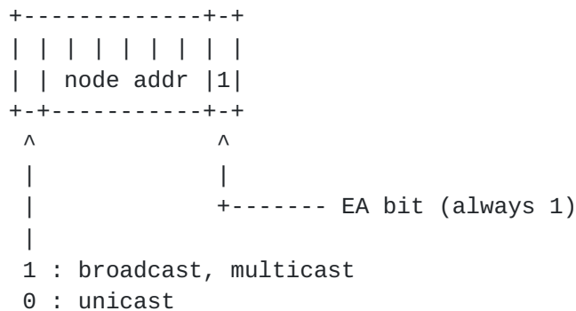
Figure 3 Address format
