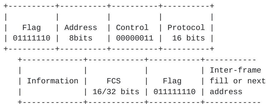
Figure 2. Frame format
