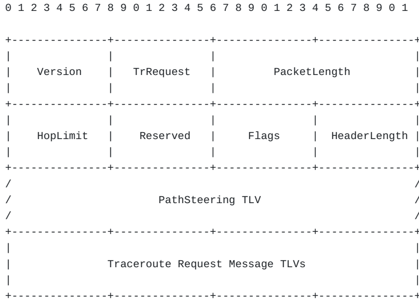
Traceroute Request CCNx Packet Format
