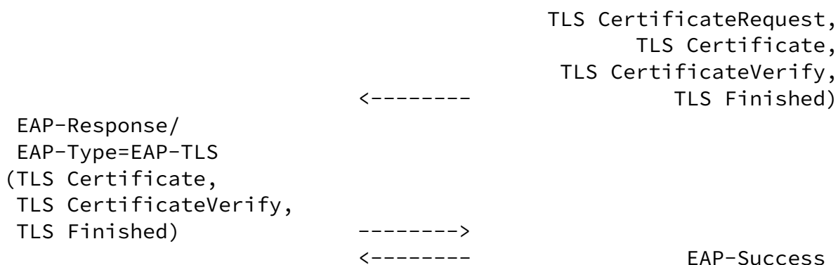
Figure 7: EAP-TLS privacy
