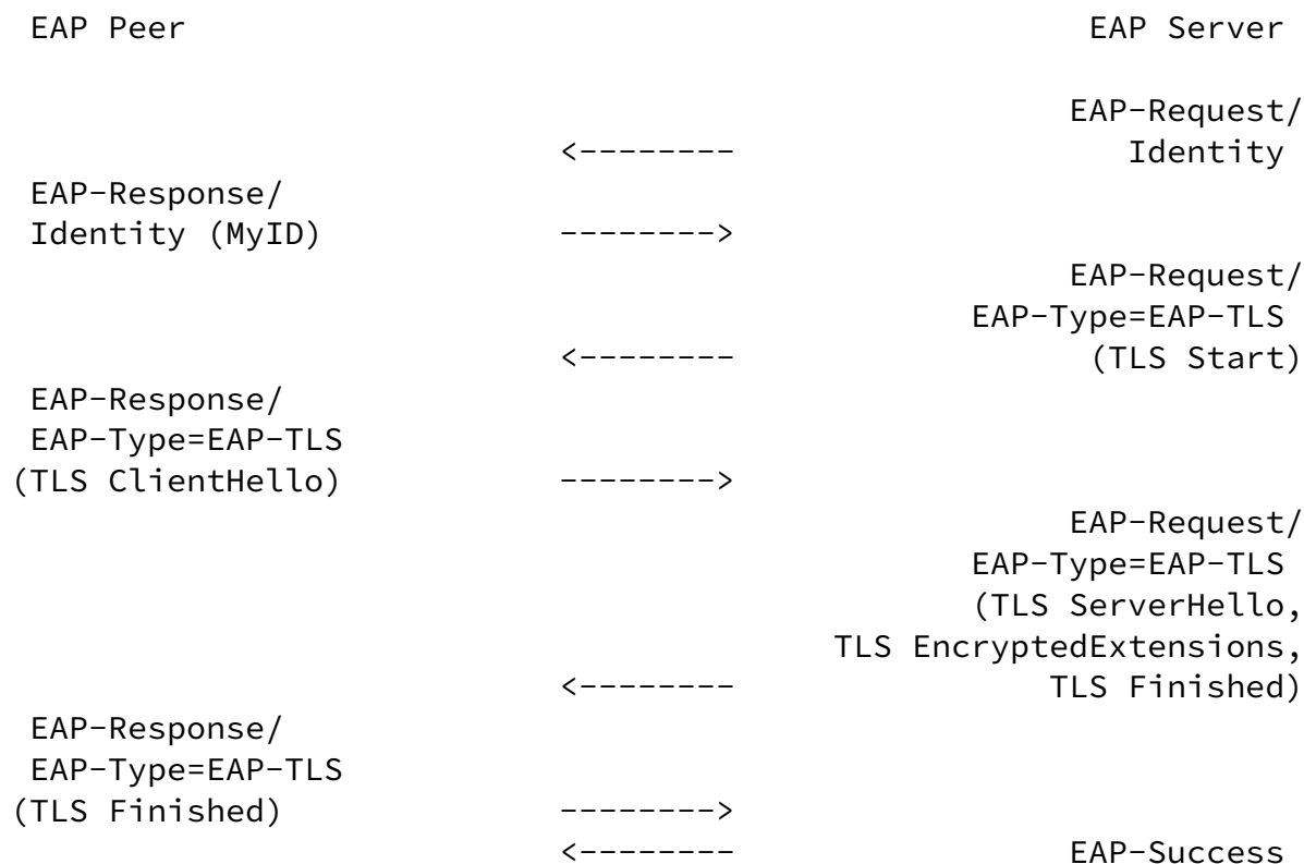
Figure 3: EAP-TLS resumption
