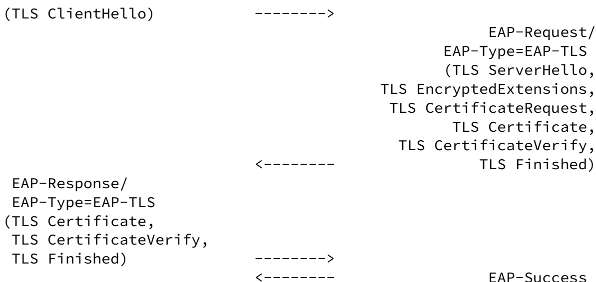
Figure 1: EAP-TLS mutual authentication
