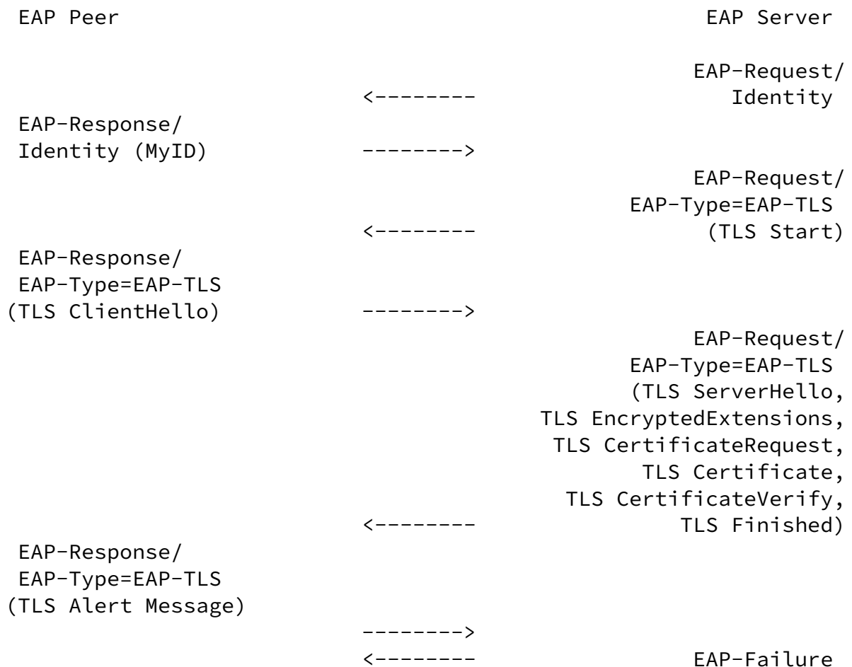
Figure 5: EAP-TLS unsuccessful server authentication
