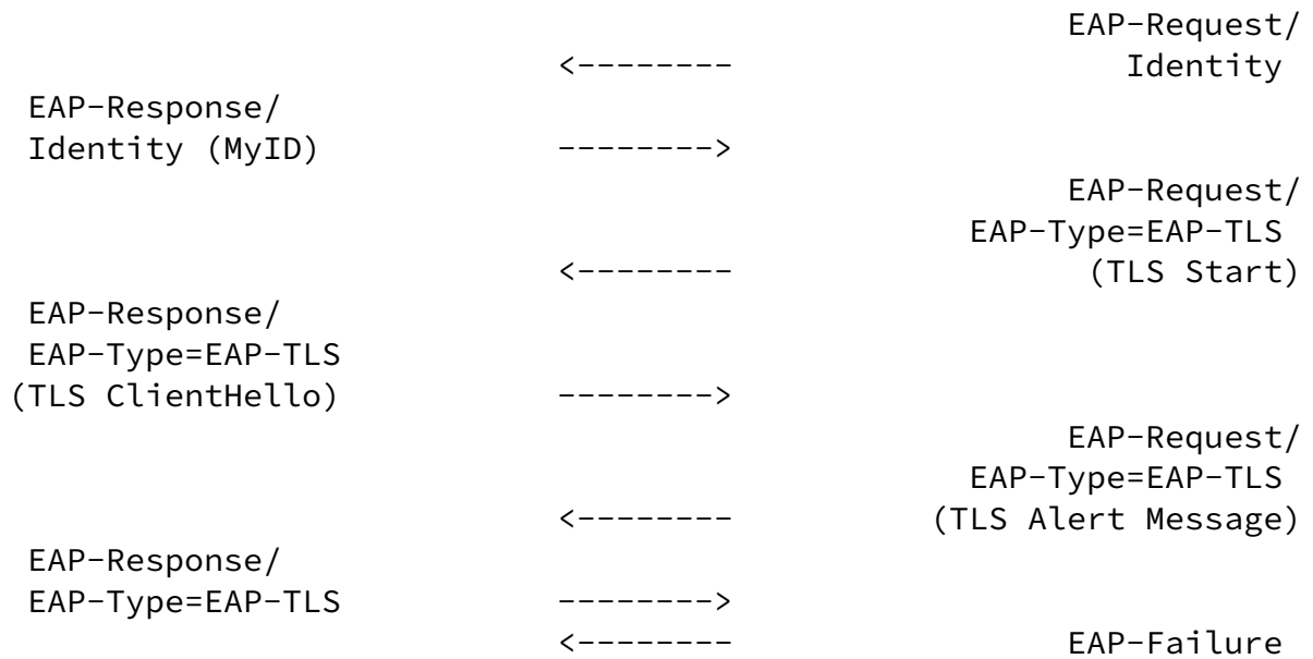
Figure 4: EAP-TLS server rejection of ClientHello
