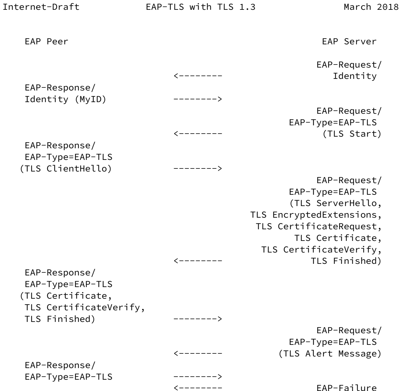
Figure 6: EAP-TLS unsuccessful client authentication
