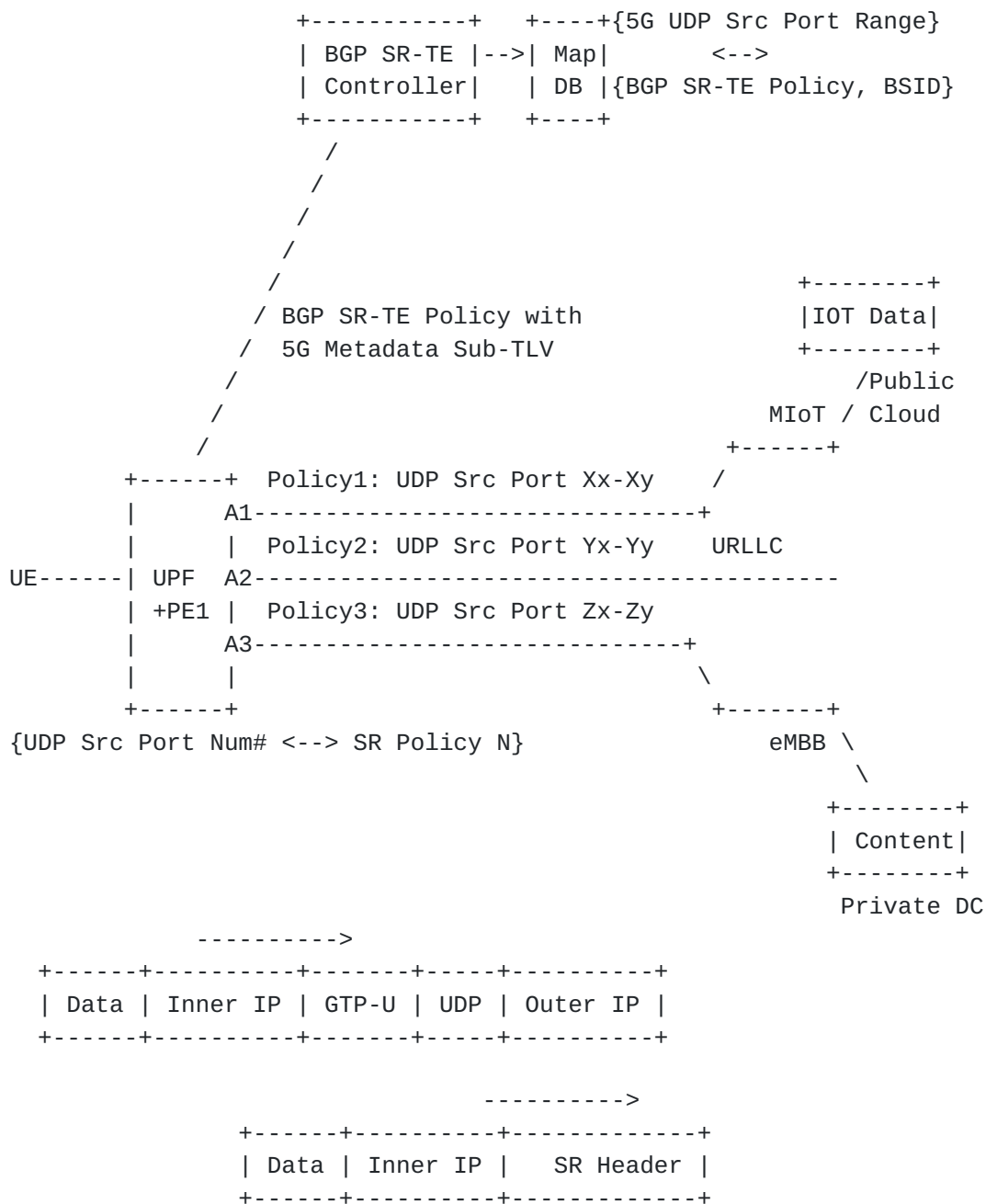
Figure 3: TN Aware Mobility Traffic Mapping to BGP SR-TE Policy Path
