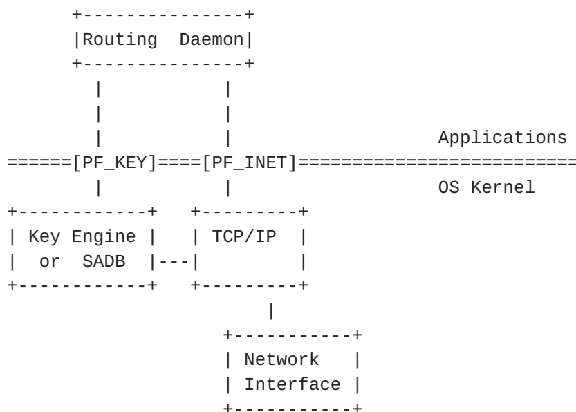
Figure 2: Relationship of Trusted Application to PF_KEY
