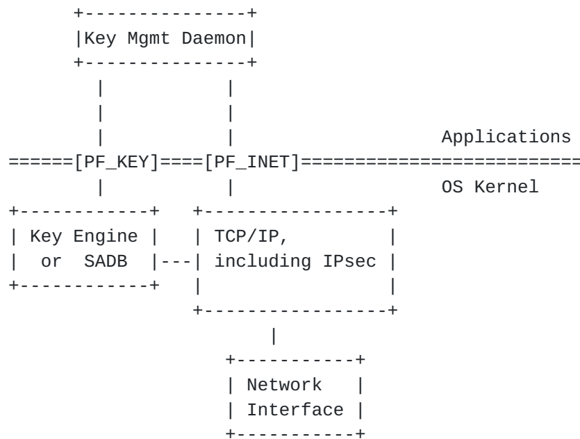
Figure 1: Relationship of Key Mgmt to PF_KEY
