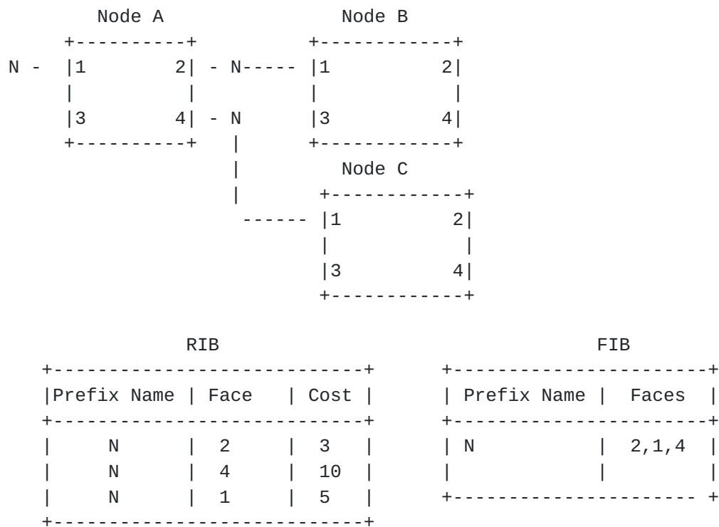
Figure 1: RIB and FIB Management, node A.
