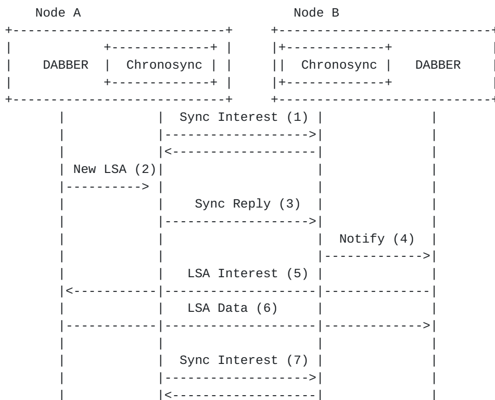
Figure 5: LSA exchange process.
